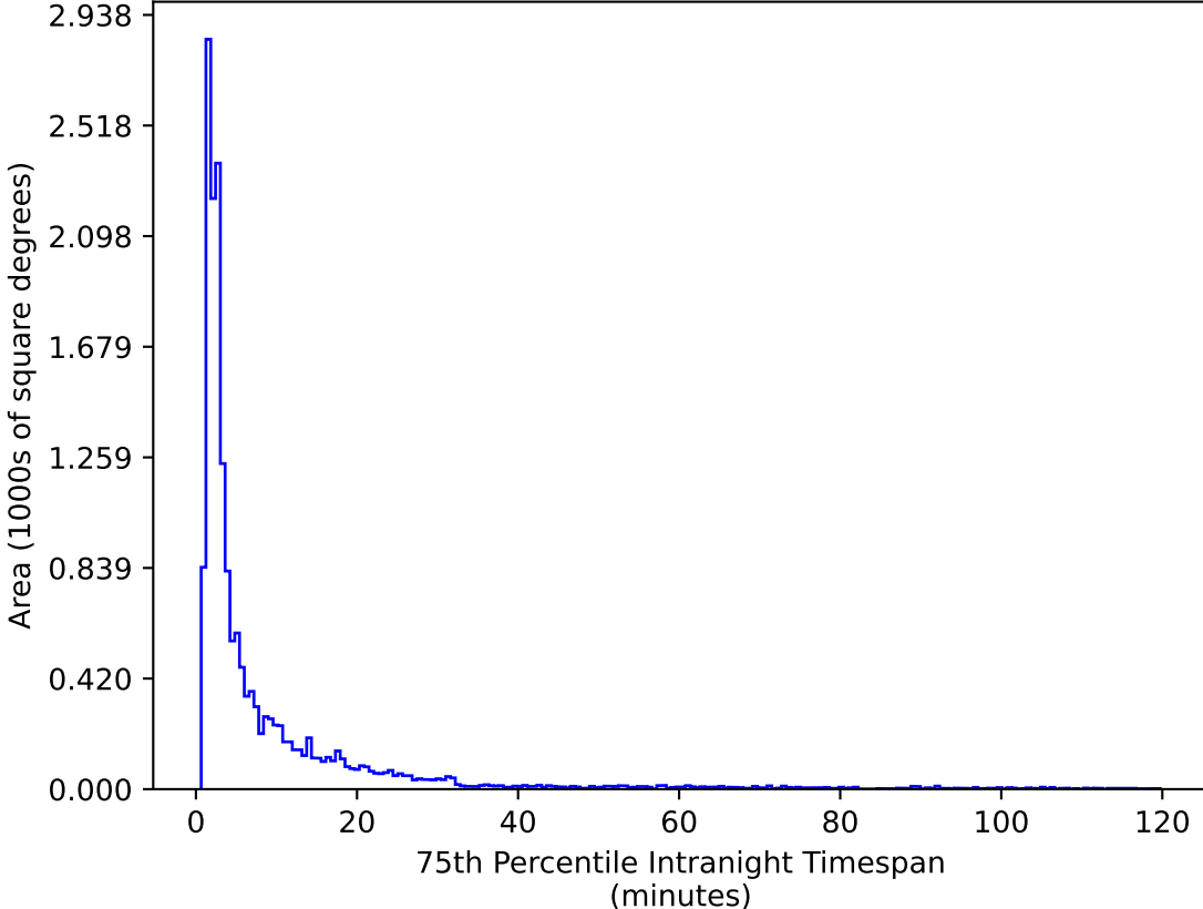
too_elab_r32_d3_ugrizy_v3.4_10yrs WFD g band: 75th Percentile Intranight Timespan
