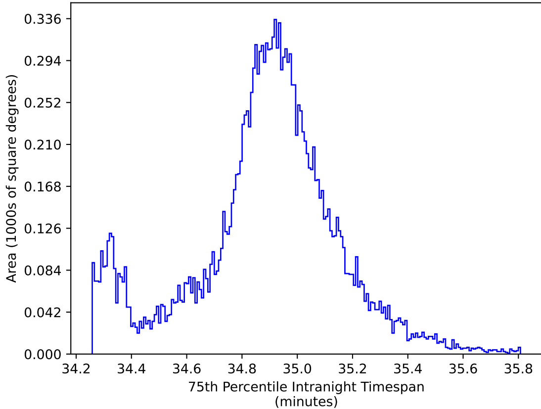
too_elab_r32_d3_ugrizy_v3.4_10yrs WFD all bands: 75th Percentile Intranight Timespan
