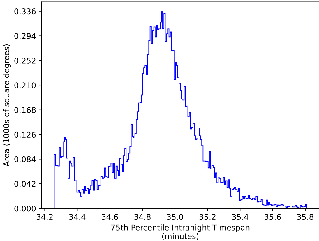
too_elab_r32_d3_ugrizy_v3.4_10yrs WFD: 75th Percentile Intranight Timespan
