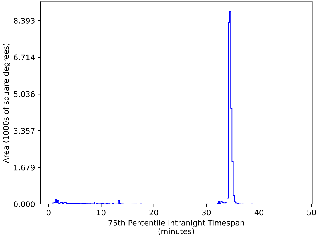
too_elab_r32_d3_ugrizy_v3.4_10yrs All sky zy bands: 75th Percentile Intranight Timespan
