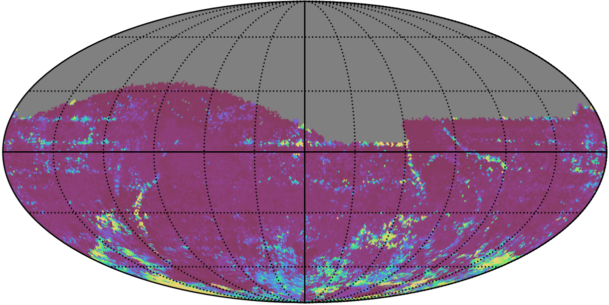
too_elab_r32_d3_ugrizy_v3.4_10yrs All sky z band: 75th Percentile Intranight Timespan
