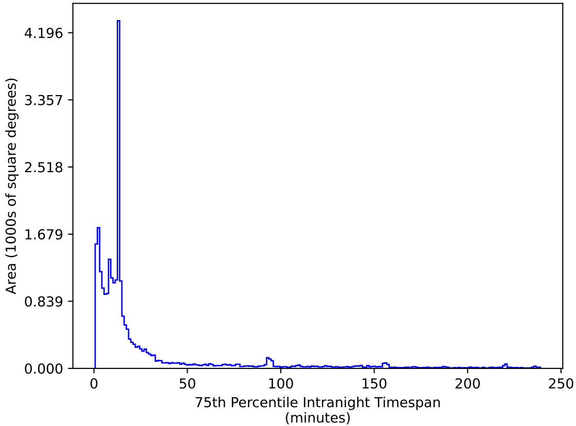
too_elab_r32_d3_ugrizy_v3.4_10yrs All sky z band: 75th Percentile Intranight Timespan
