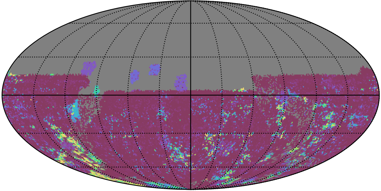
too_elab_r32_d3_ugrizy_v3.4_10yrs All sky u band: 75th Percentile Intranight Timespan
