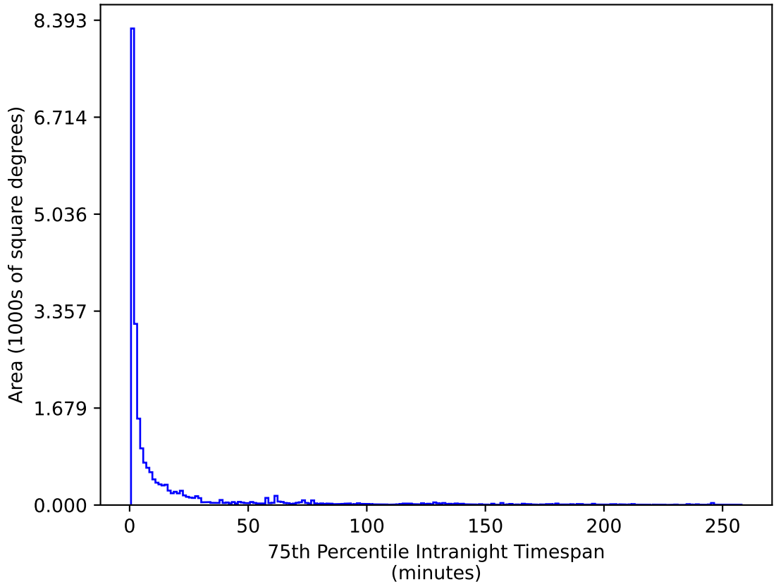
too_elab_r32_d3_ugrizy_v3.4_10yrs All sky u band: 75th Percentile Intranight Timespan
