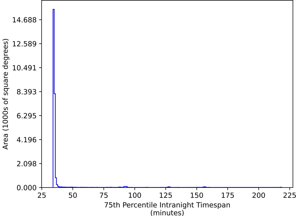
too_elab_r32_d3_ugrizy_v3.4_10yrs All sky ri bands: 75th Percentile Intranight Timespan
