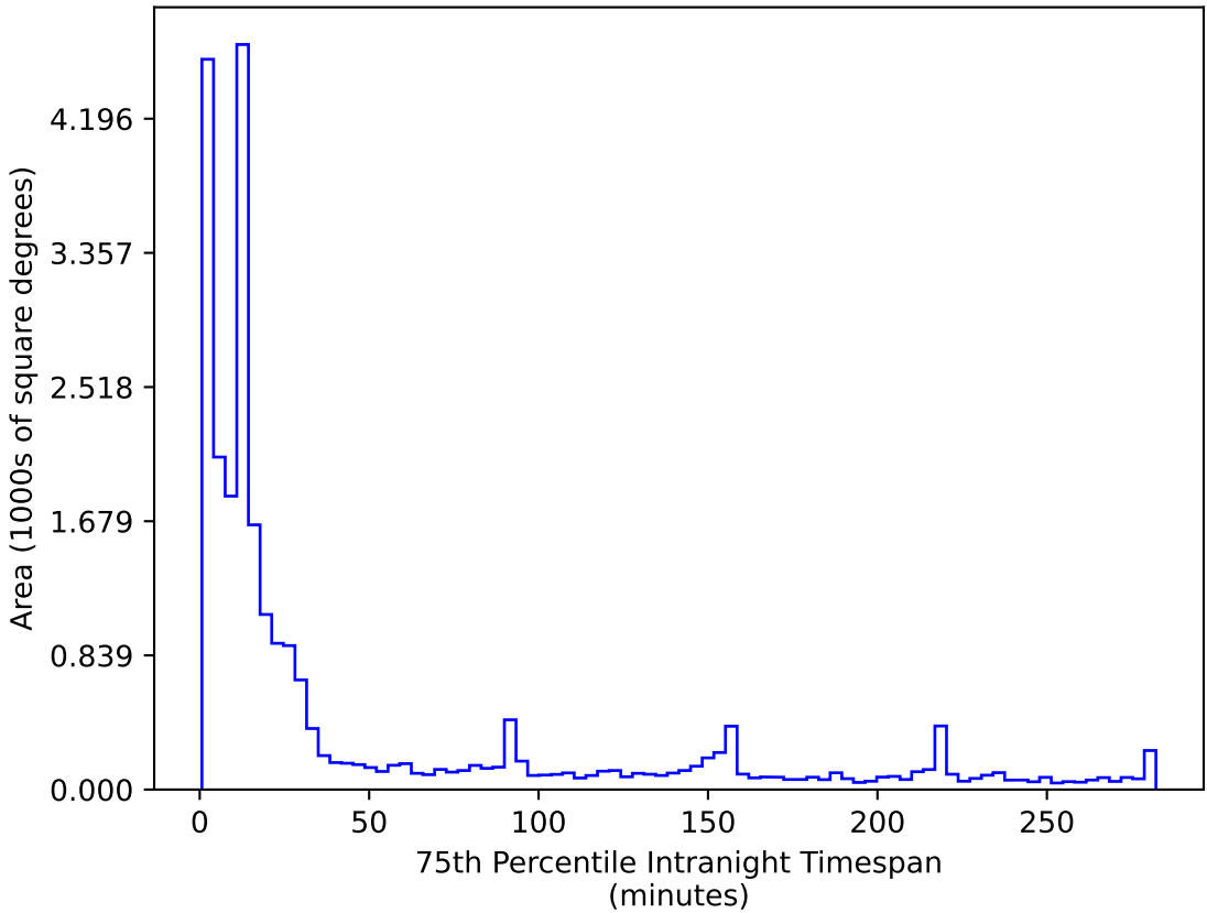
too_elab_r32_d3_ugrizy_v3.4_10yrs All sky r band: 75th Percentile Intranight Timespan
