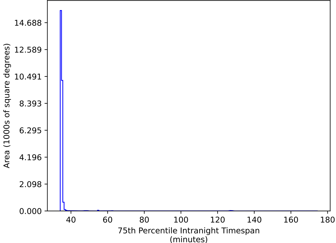
too_elab_r32_d3_ugrizy_v3.4_10yrs All sky iz bands: 75th Percentile Intranight Timespan
