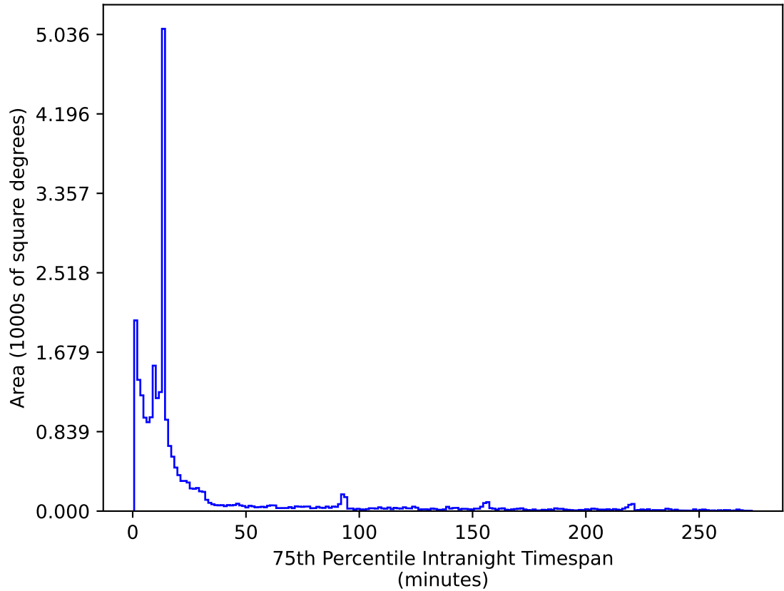
too_elab_r32_d3_ugrizy_v3.4_10yrs All sky i band: 75th Percentile Intranight Timespan
