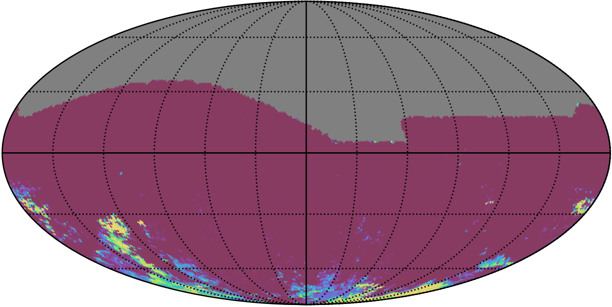
too_elab_r32_d3_ugrizy_v3.4_10yrs All sky gr bands: 75th Percentile Intranight Timespan
