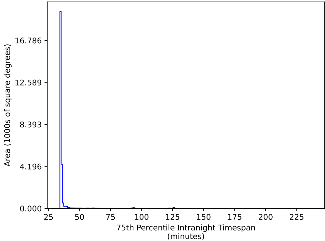
too_elab_r32_d3_ugrizy_v3.4_10yrs All sky gr bands: 75th Percentile Intranight Timespan
