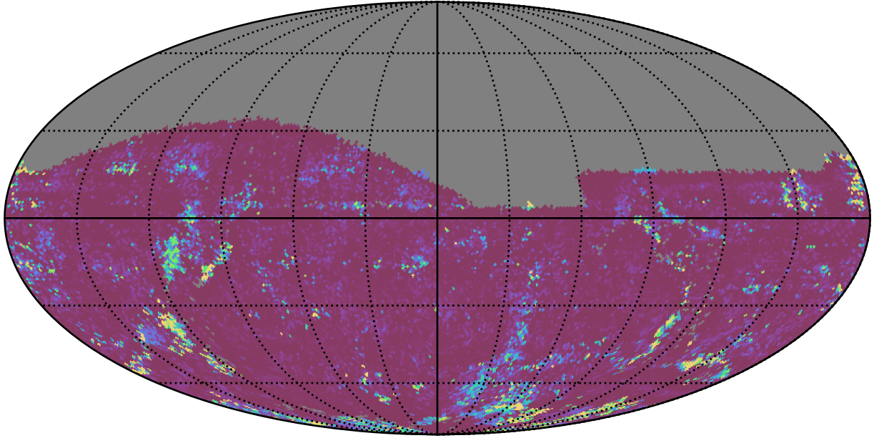
too_elab_r32_d3_ugrizy_v3.4_10yrs All sky g band: 75th Percentile Intranight Timespan
