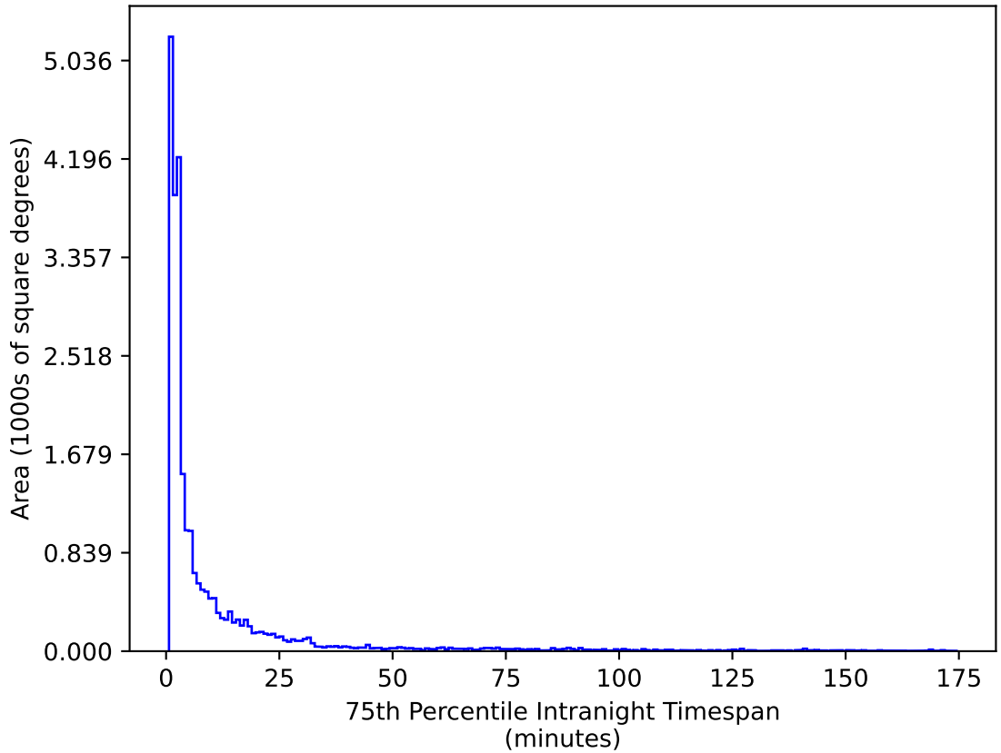
too_elab_r32_d3_ugrizy_v3.4_10yrs All sky g band: 75th Percentile Intranight Timespan
