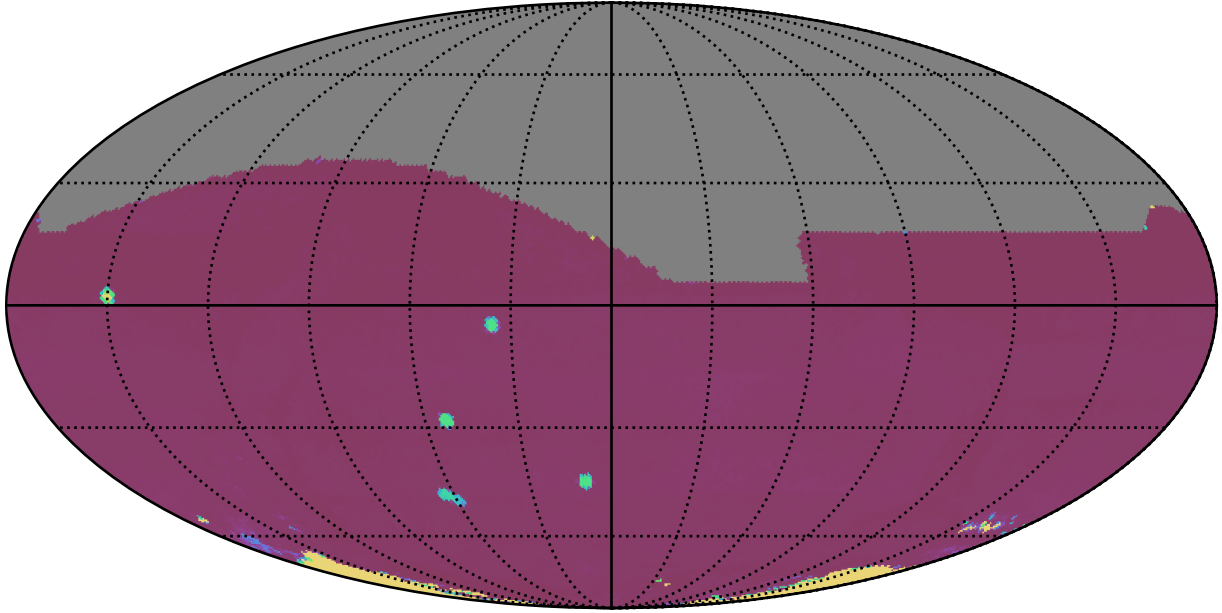
too_elab_r32_d3_ugrizy_v3.4_10yrs All sky all bands: 75th Percentile Intranight Timespan
