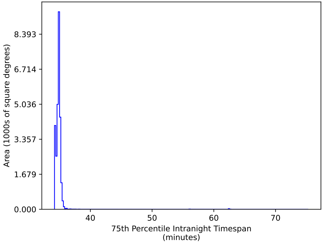
too_elab_r32_d3_ugrizy_v3.4_10yrs All sky: 75th Percentile Intranight Timespan
