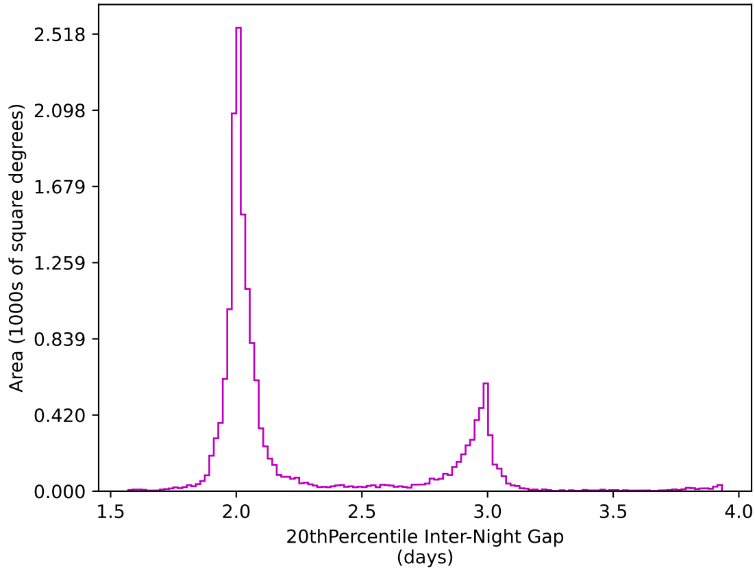
too_elab_r32_d3_ugrizy_v3.4_10yrs WFD z band: 20thPercentile Inter-Night Gap
