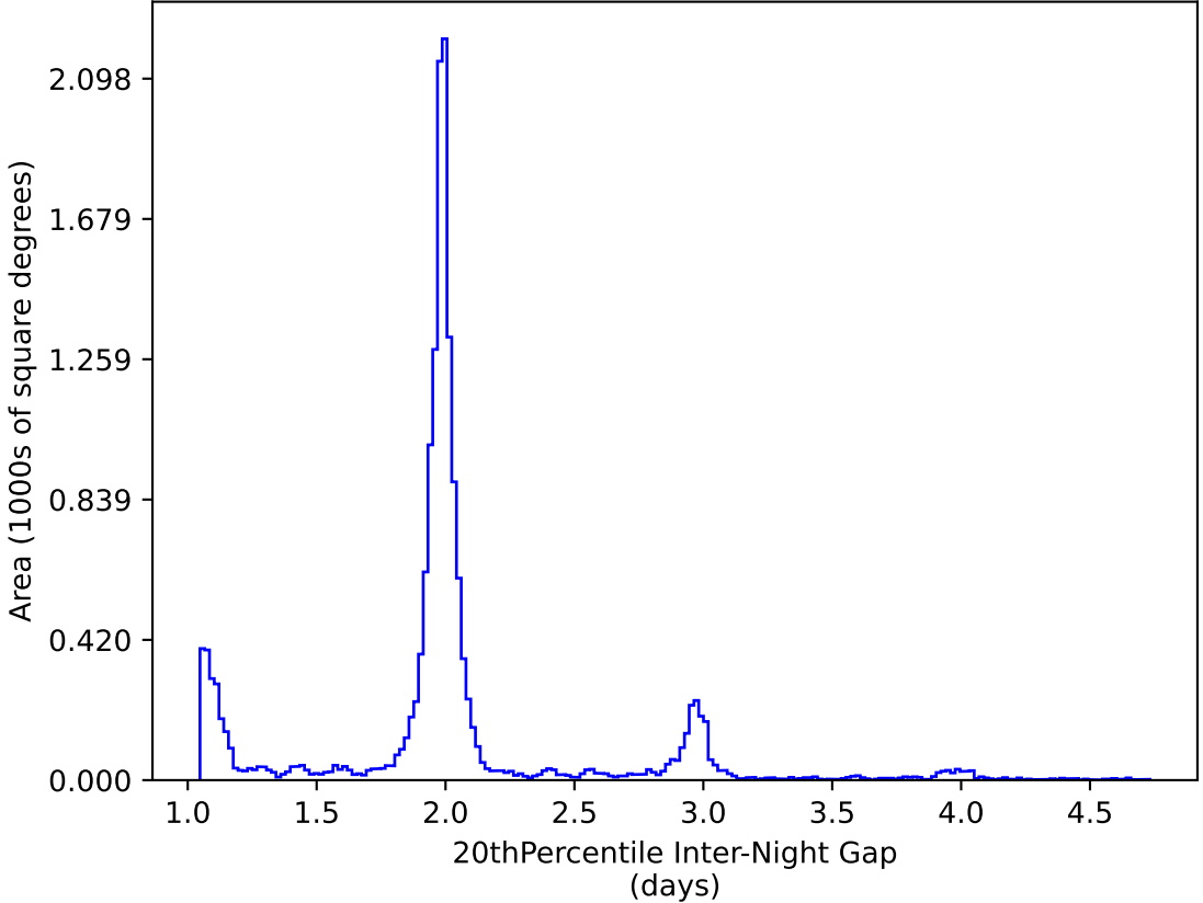
too_elab_r32_d3_ugrizy_v3.4_10yrs WFD y band: 20thPercentile Inter-Night Gap
