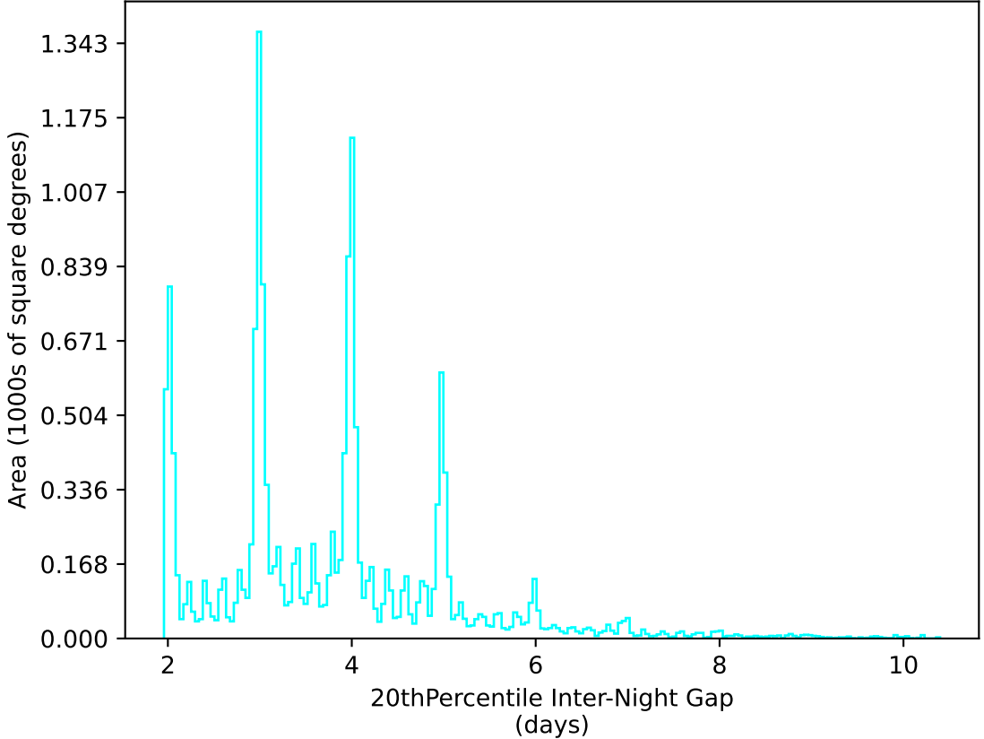
too_elab_r32_d3_ugrizy_v3.4_10yrs WFD u band: 20thPercentile Inter-Night Gap
