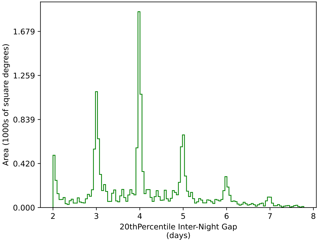
too_elab_r32_d3_ugrizy_v3.4_10yrs WFD g band: 20thPercentile Inter-Night Gap
