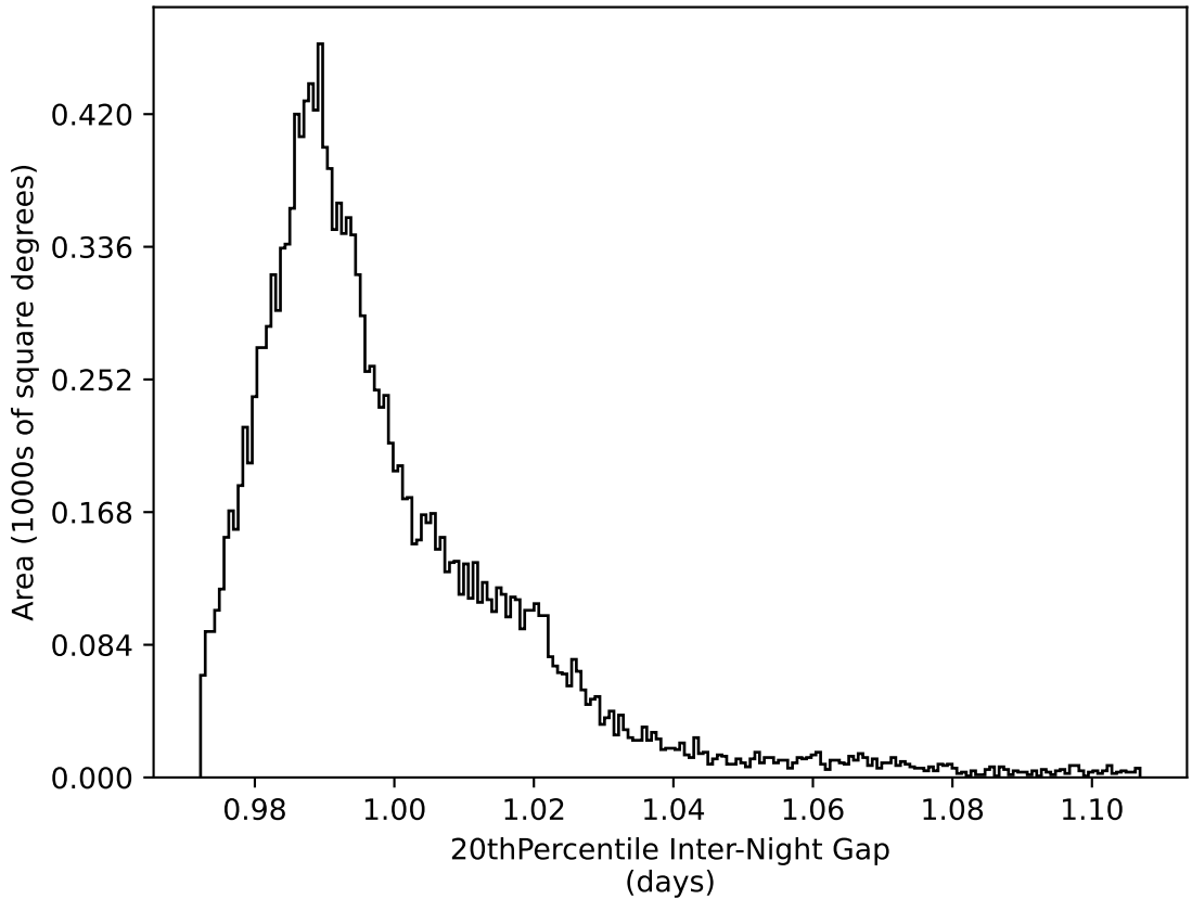
too_elab_r32_d3_ugrizy_v3.4_10yrs WFD all bands: 20thPercentile Inter-Night Gap
