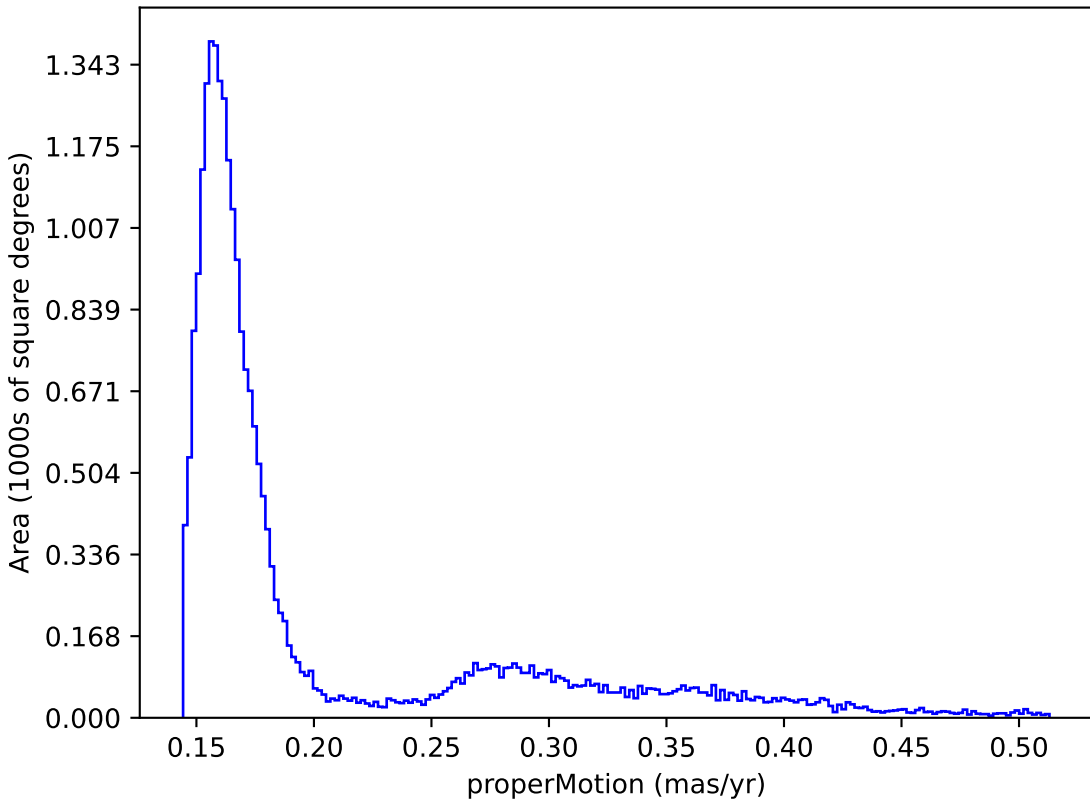
too_elab_r32_d3_ugrizy_v3.4_10yrs : properMotion
