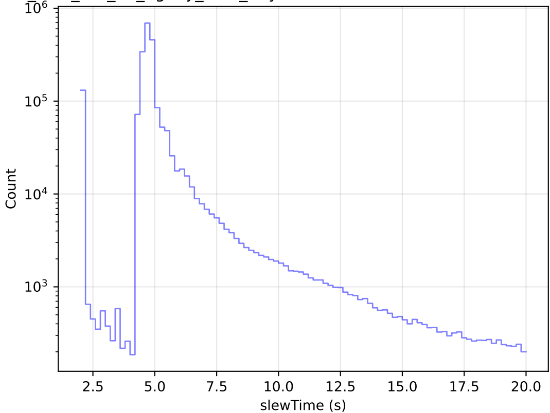
too_elab_r32_d3_ugrizy_v3.4_10yrs All visits: Zoom Slew Time Histogram
