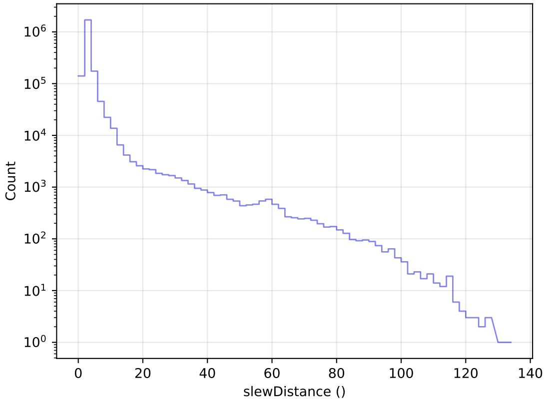
too_elab_r32_d3_ugrizy_v3.4_10yrs All visits: Slew Distance Histogram
