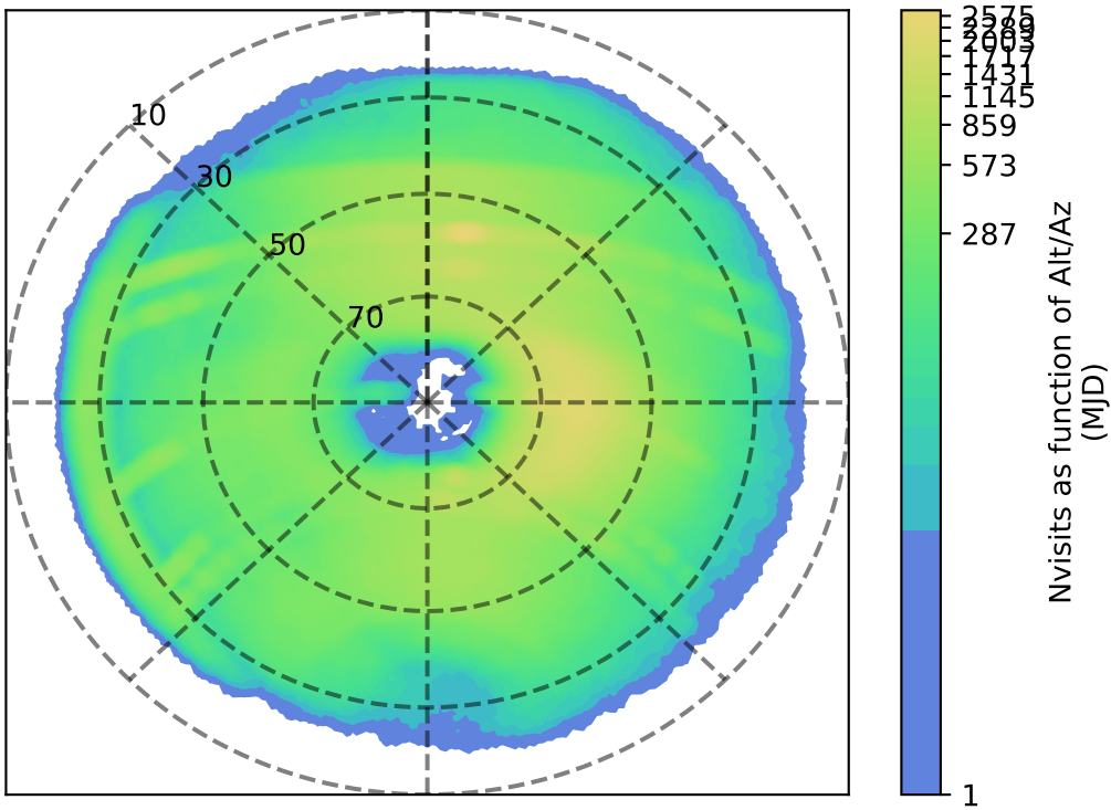
too_elab_r32_d3_ugrizy_v3.4_10yrs r: Nvisits as function of Alt/Az
