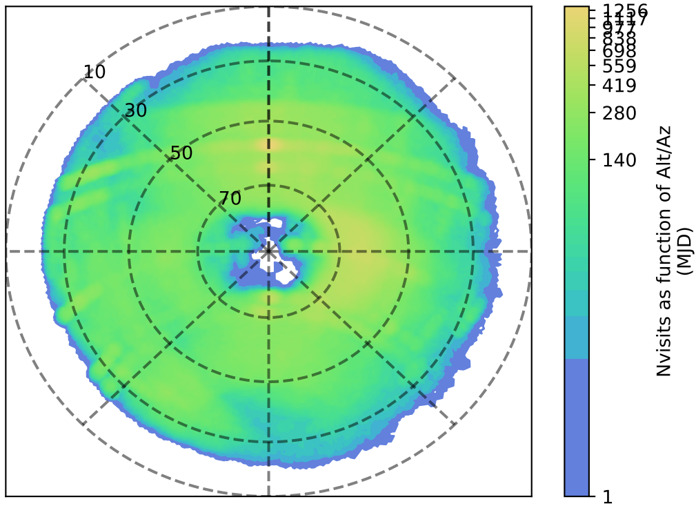
too_elab_r32_d3_ugrizy_v3.4_10yrs g: Nvisits as function of Alt/Az
