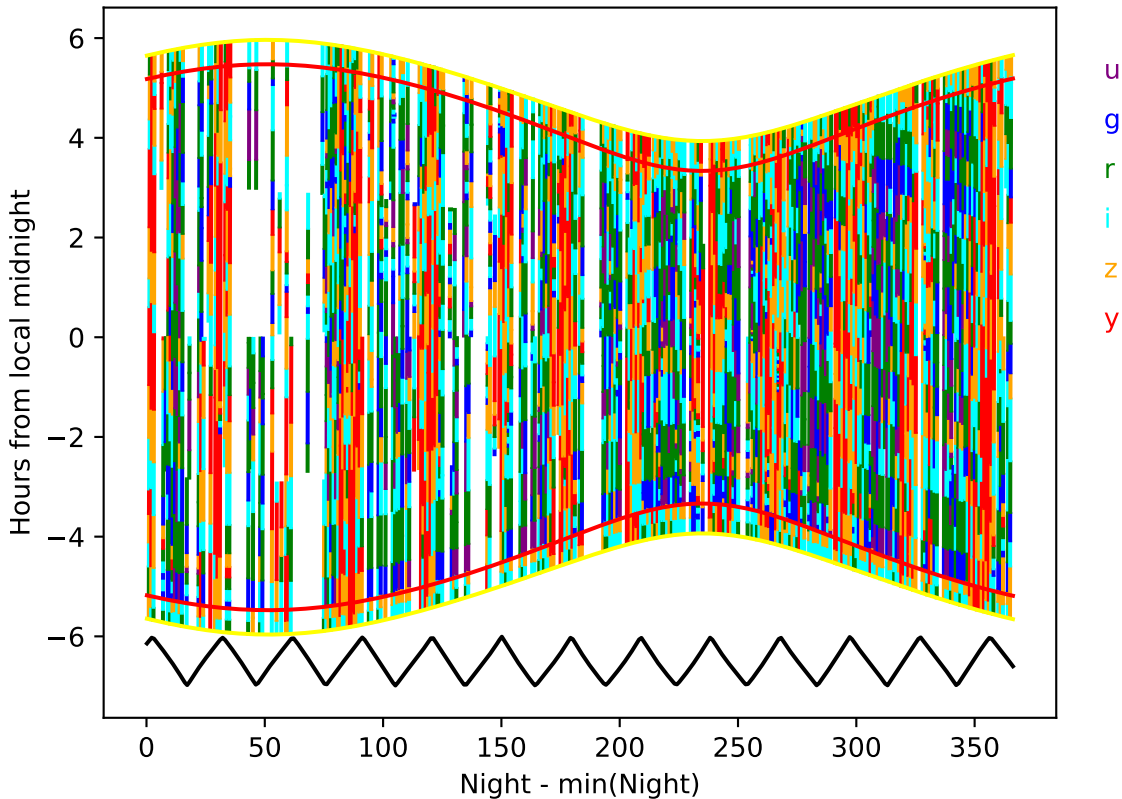
too_elab_r32_d3_ugrizy_v3.4_10yrs year 9-10: Hourglass
