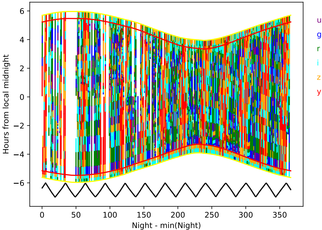
too_elab_r32_d3_ugrizy_v3.4_10yrs year 6-7: Hourglass
