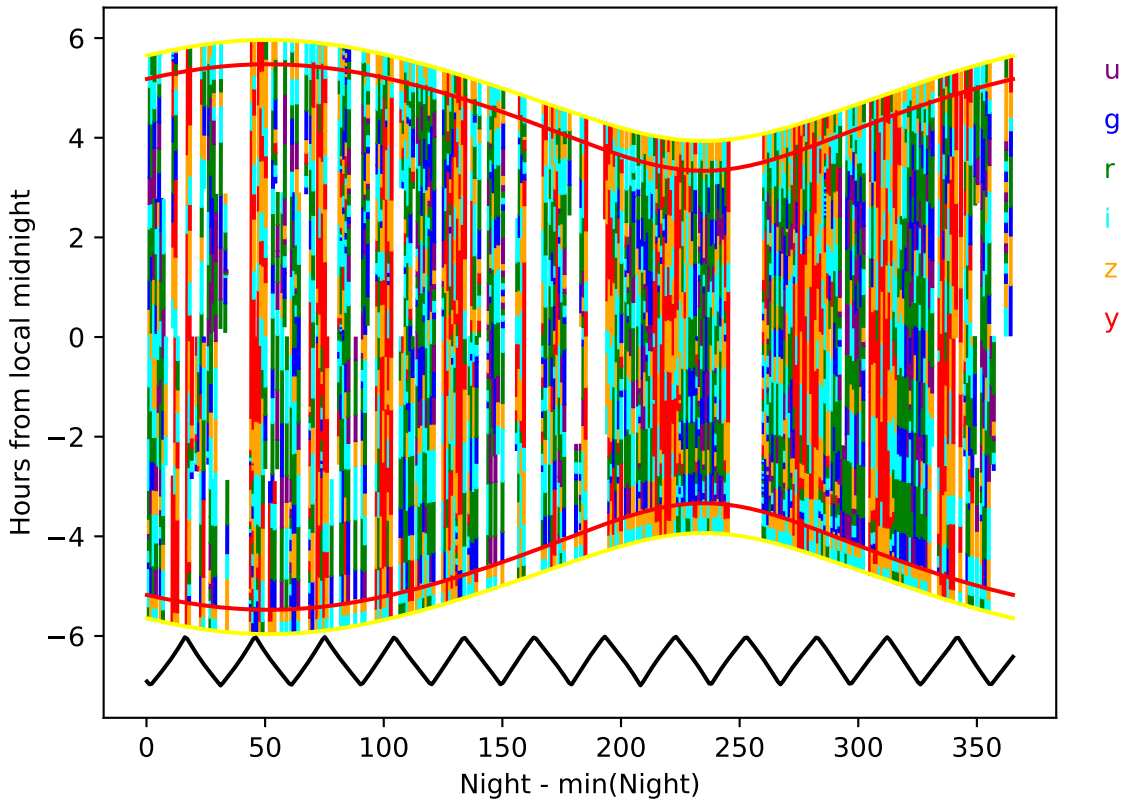
too_elab_r32_d3_ugrizy_v3.4_10yrs year 5-6: Hourglass
