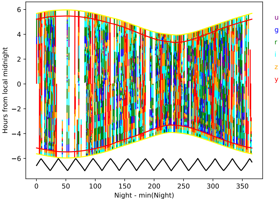
too_elab_r32_d3_ugrizy_v3.4_10yrs_year 3-4: Hourglass
