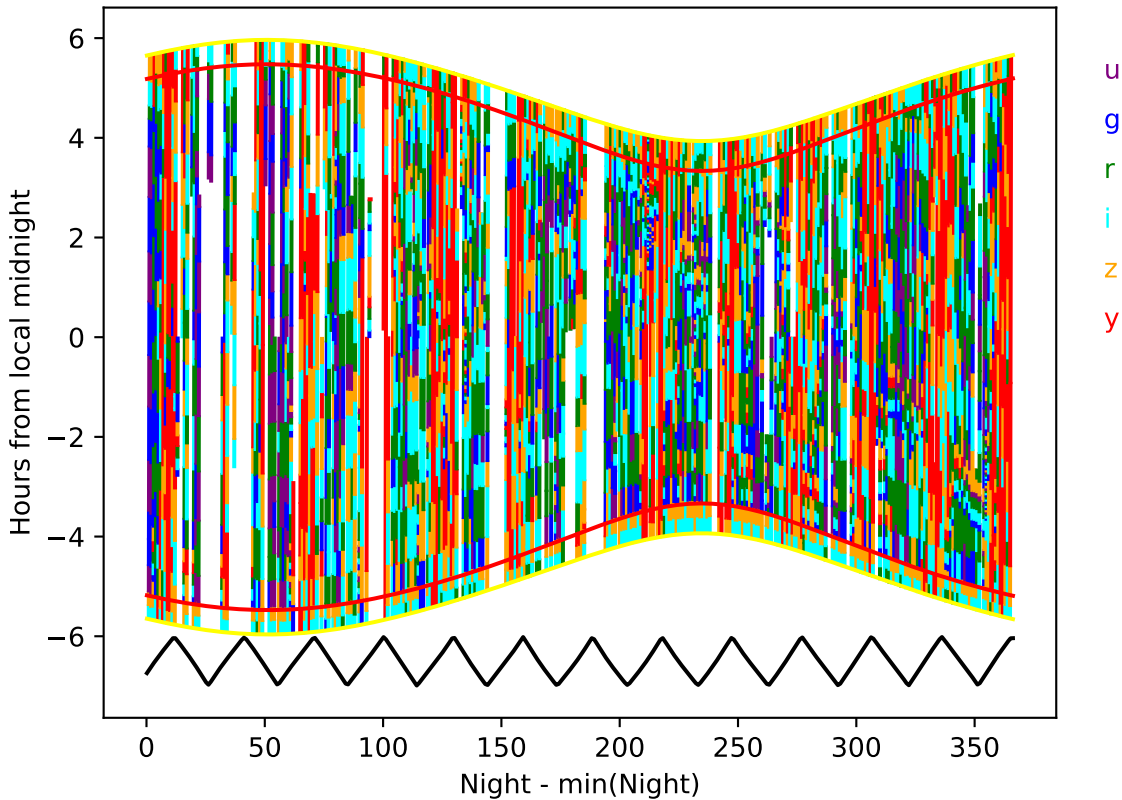
too_elab_r32_d3_ugrizy_v3.4_10yrs_year 0-1: Hourglass
