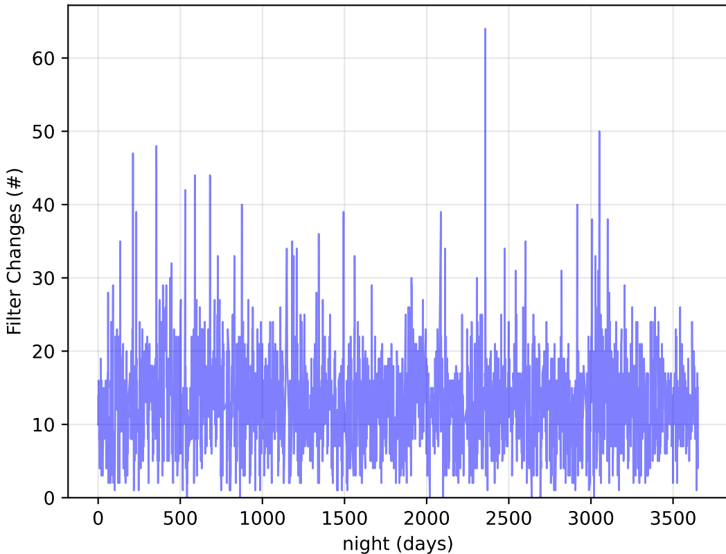
too_elab_r32_d3_ugrizy_v3.4_10yrs : Filter Changes
