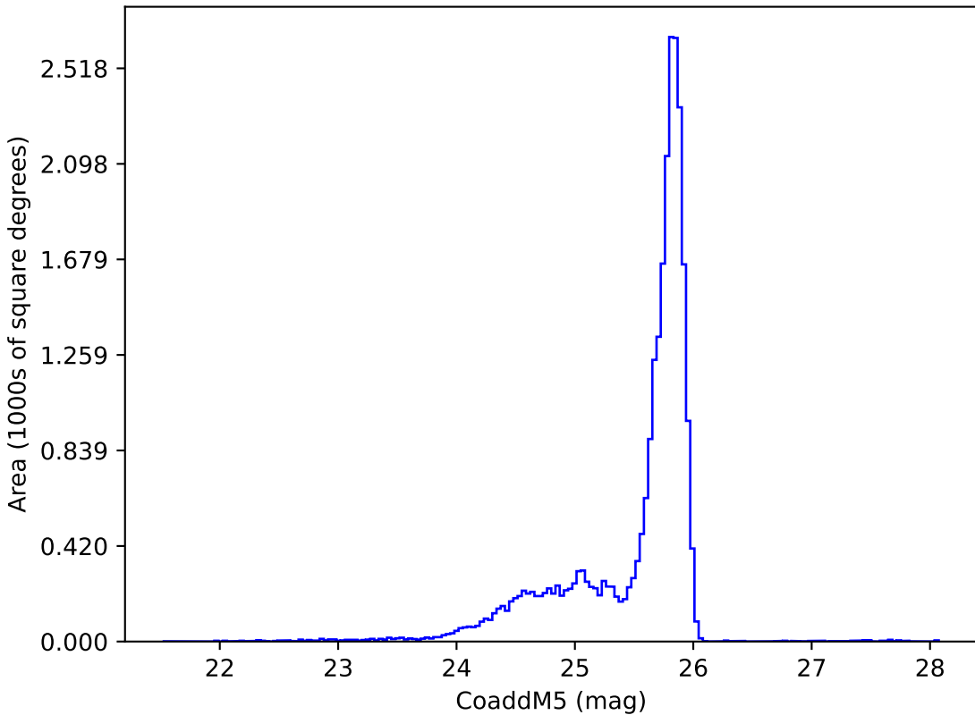
too_elab_r32_d3_ugrizy_v3.4_10yrs z: CoaddM5
