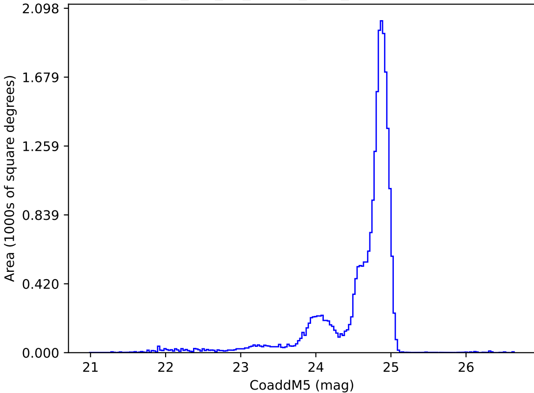
too_elab_r32_d3_ugrizy_v3.4_10yrs y: CoaddM5
