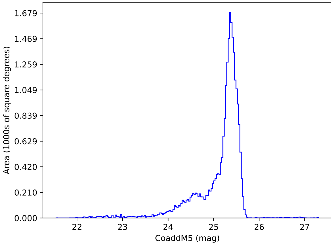
too_elab_r32_d3_ugrizy_v3.4_10yrs u: CoaddM5
