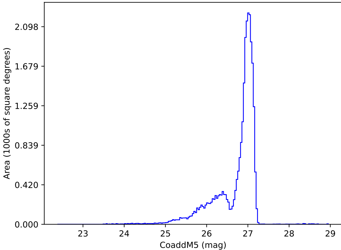
too_elab_r32_d3_ugrizy_v3.4_10yrs r: CoaddM5
