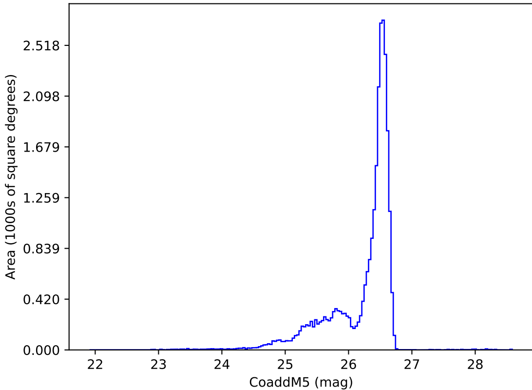
too_elab_r32_d3_ugrizy_v3.4_10yrs i: CoaddM5
