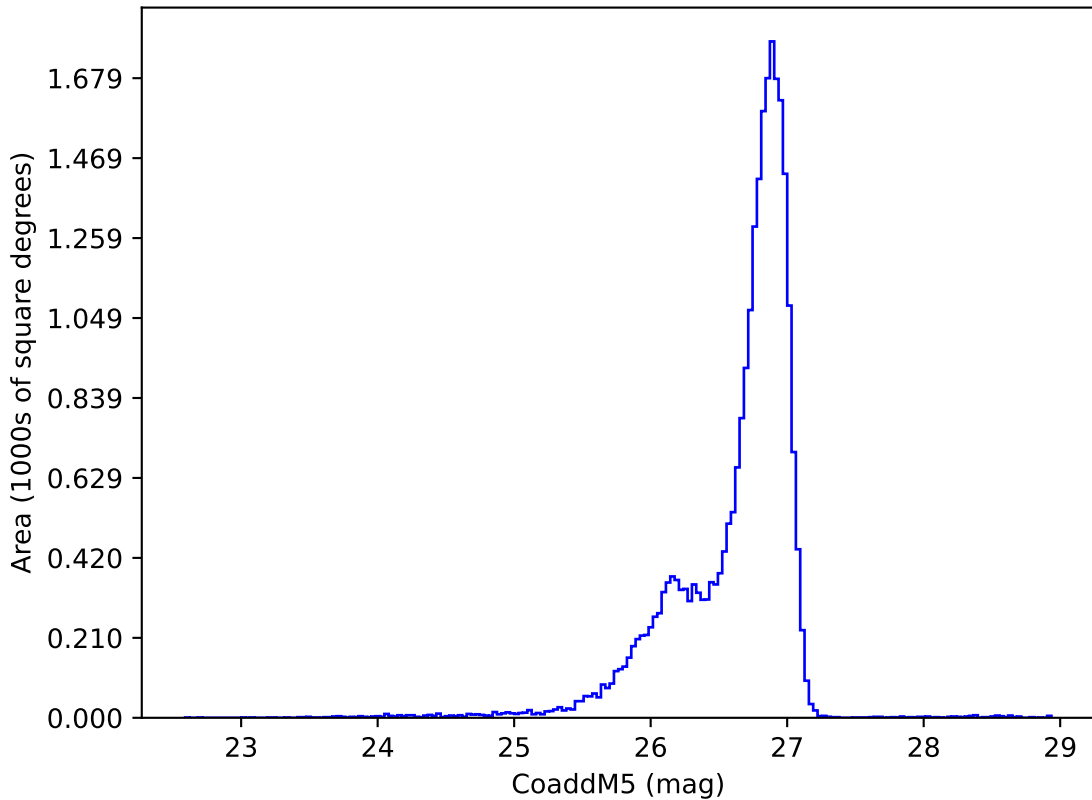
too_elab_r32_d3_ugrizy_v3.4_10yrs g: CoaddM5
