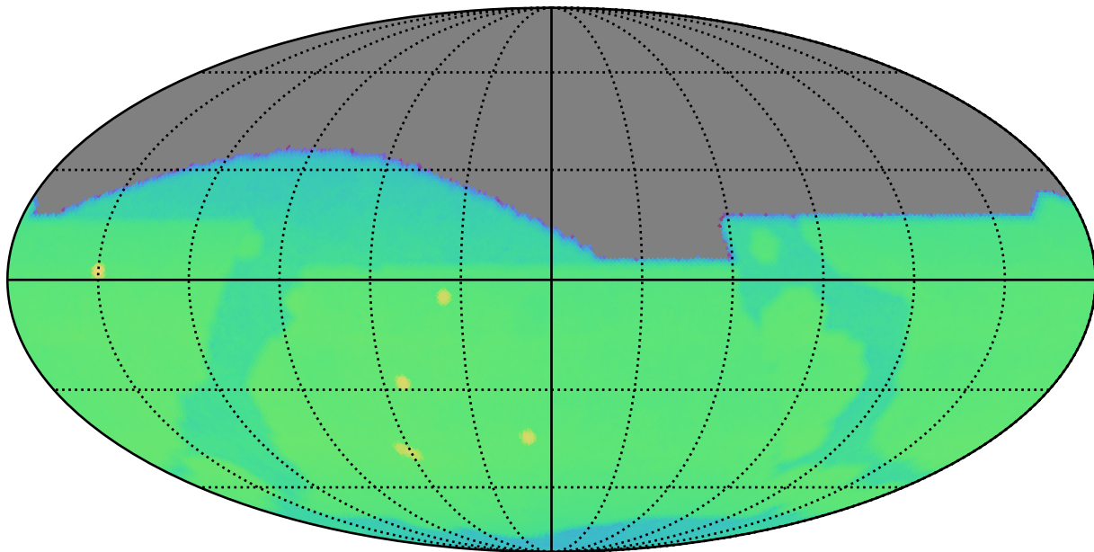
too_elab_r32_d3_ugrizy_v3.4_10yrs : CoaddM5
