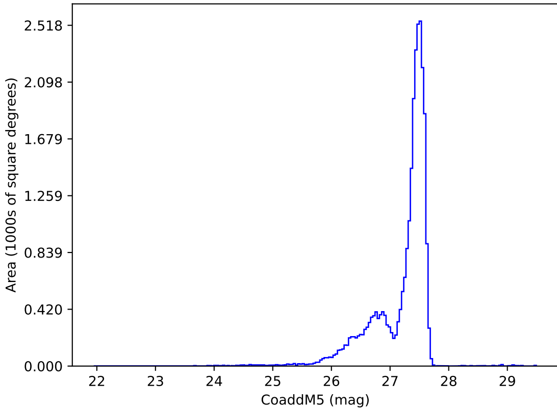
too_elab_r32_d3_ugrizy_v3.4_10yrs : CoaddM5
