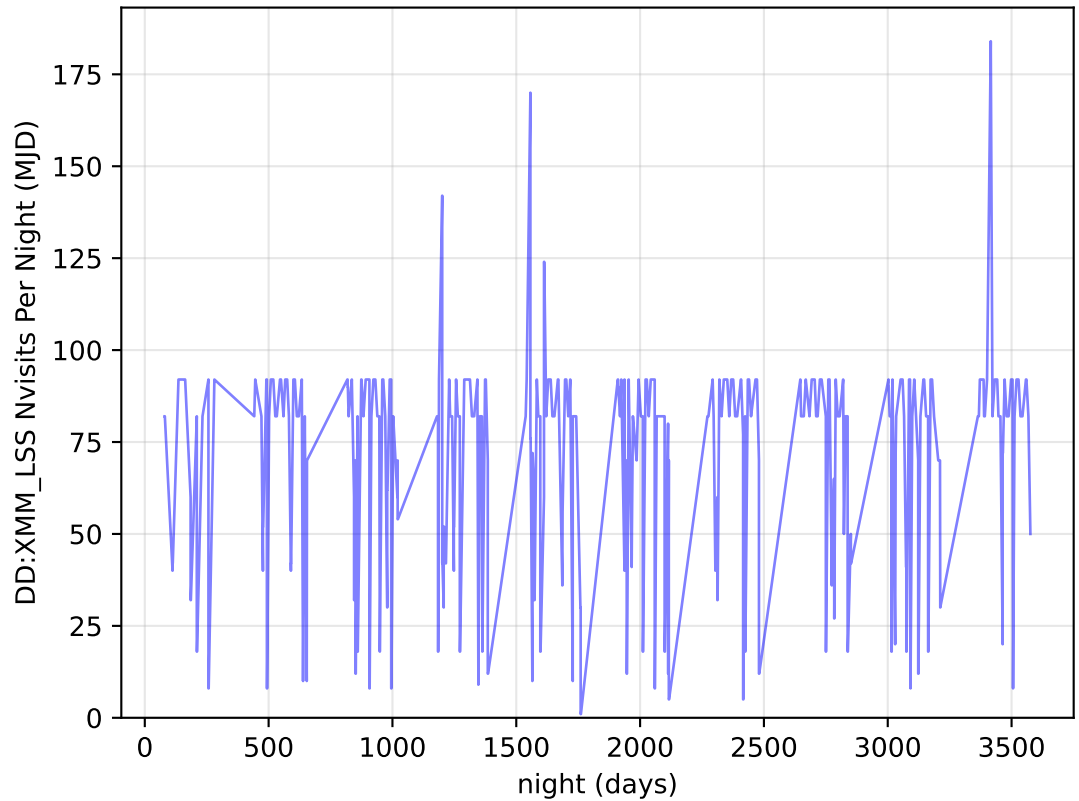
too_elab_r32_d3_ugrizy_v3.4_10yrs all bands: DD:XMM_LSS Nvisits Per Night
