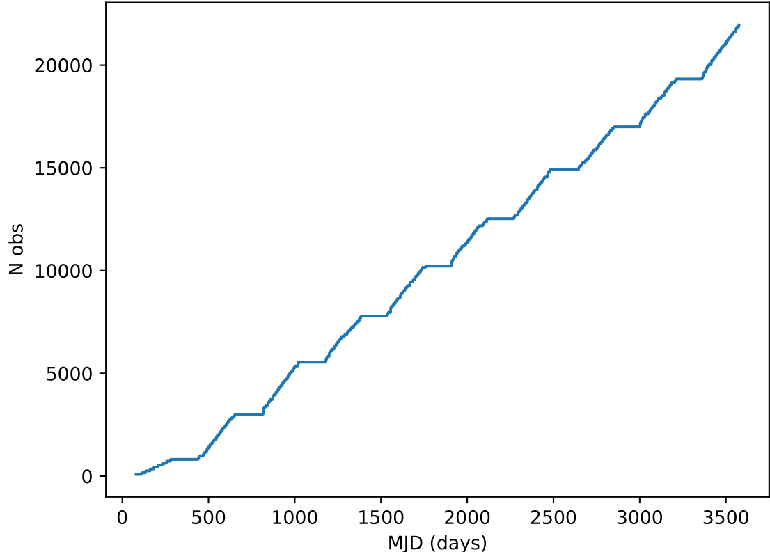
too_elab_r32_d3_ugrizy_v3.4_10yrs all bands: DD:XMM_LSS Cumulative NVisits
