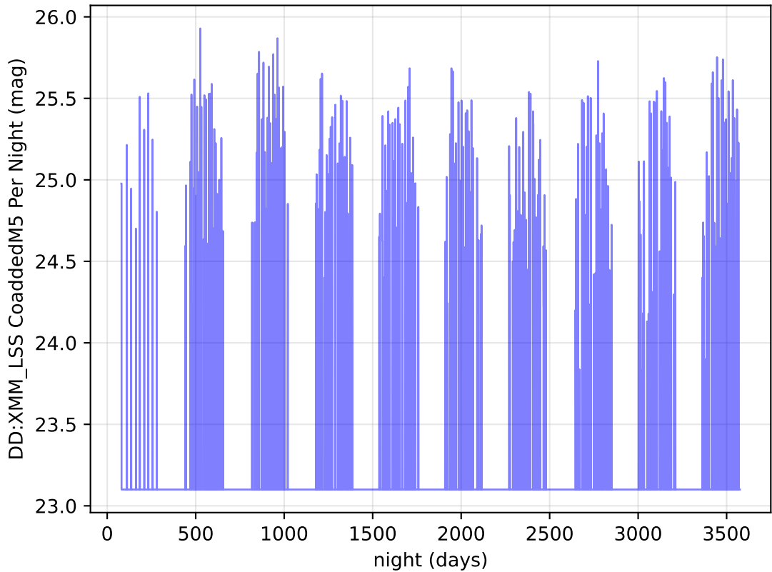
too_elab_r32_d3_ugrizy_v3.4_10yrs i band: DD:XMM_LSS CoaddedM5 Per Night
