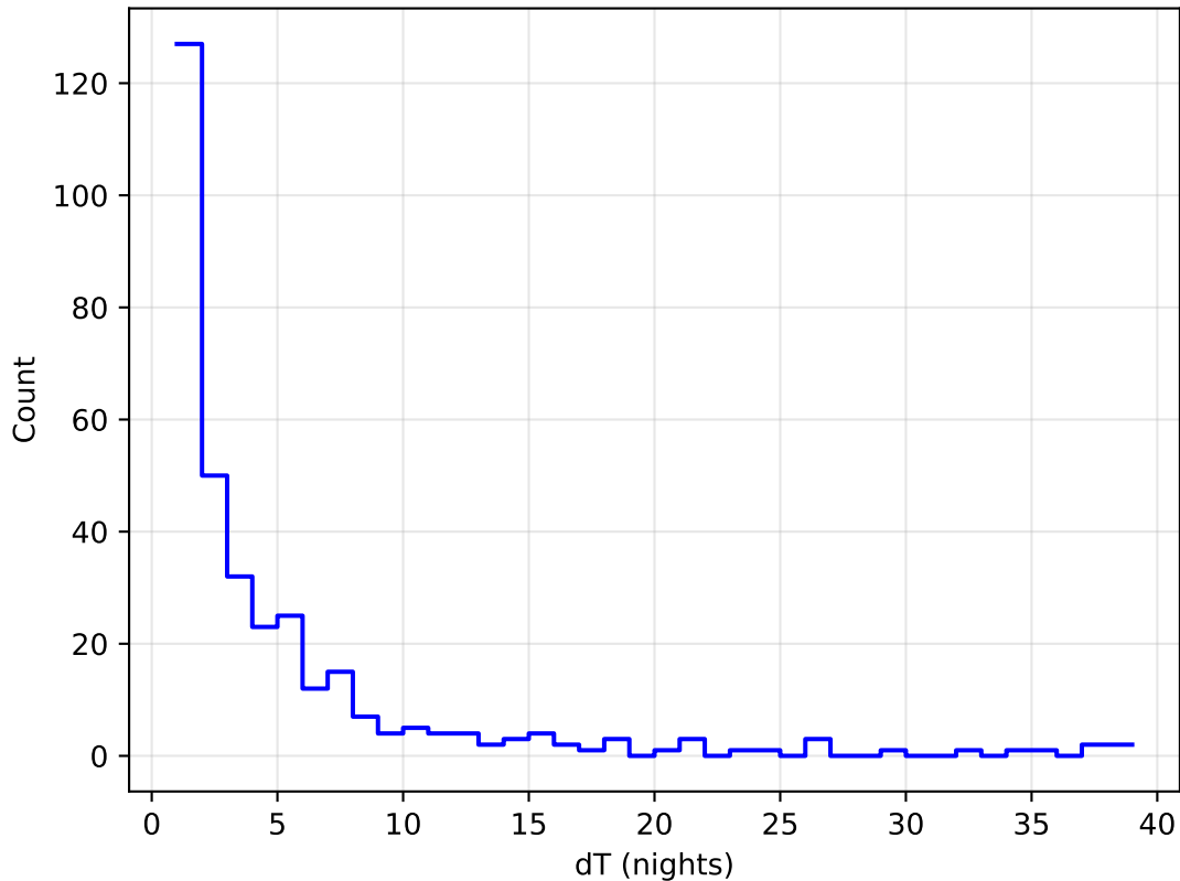
too_elab_r32_d3_ugrizy_v3.4_10yrs all bands: DD:WFD Delta Nights Histogram
