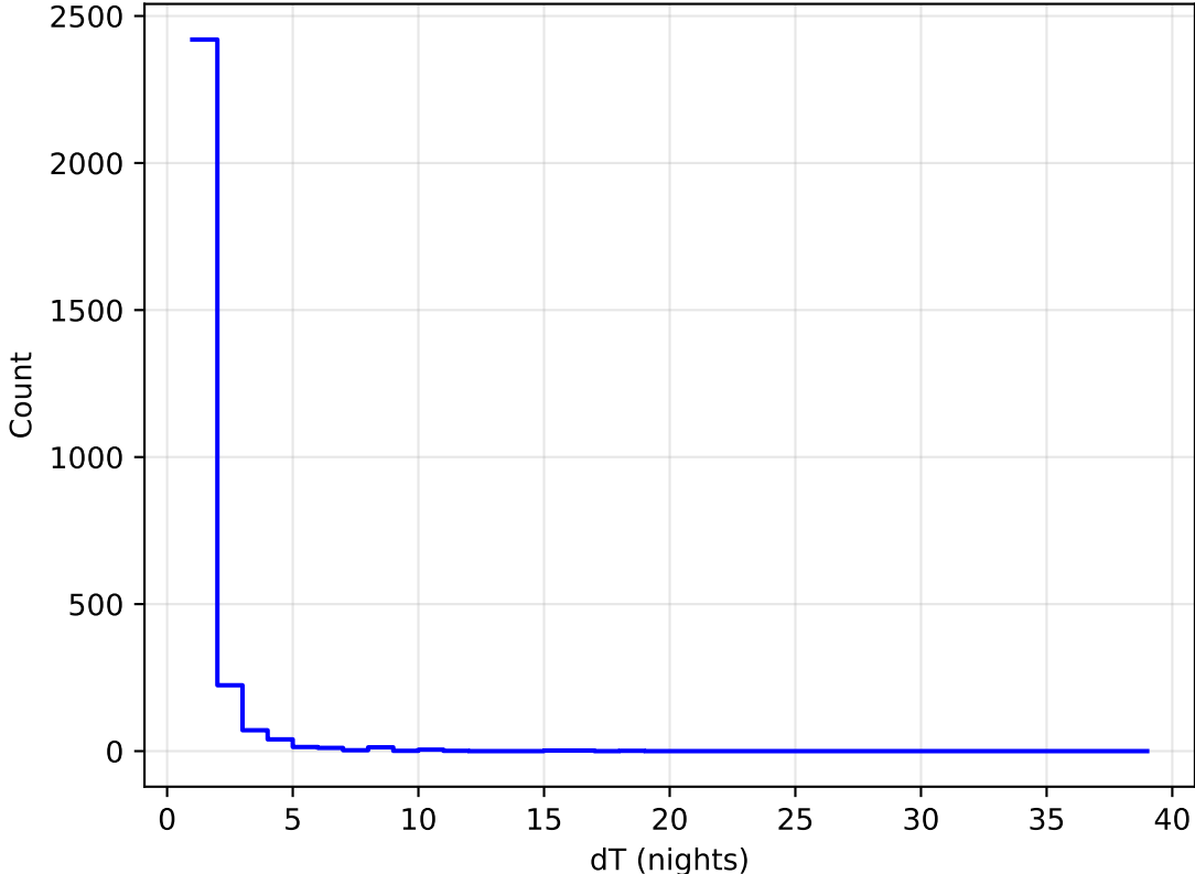
too_elab_r32_d3_ugrizy_v3.4_10yrs all bands: DD:WFD Delta Nights Histogram
