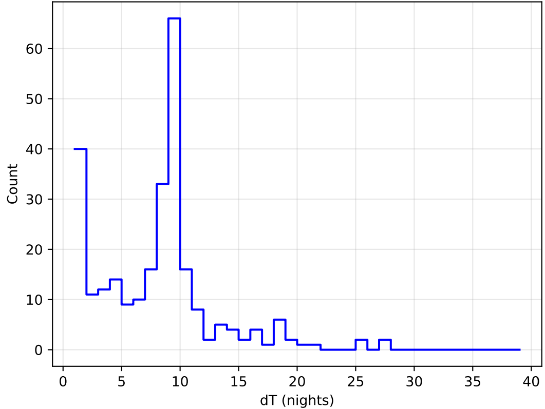
too_elab_r32_d3_ugrizy_v3.4_10yrs all bands: DD:ELAISS1 Delta Nights Histogram
