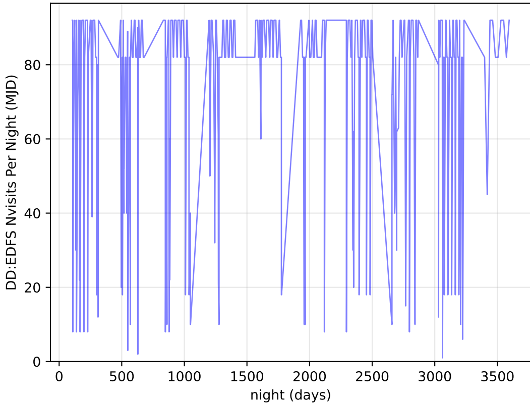
too_elab_r32_d3_ugrizyv3.4_10yrs all bands: DD:EDFS Nvisits Per Night
