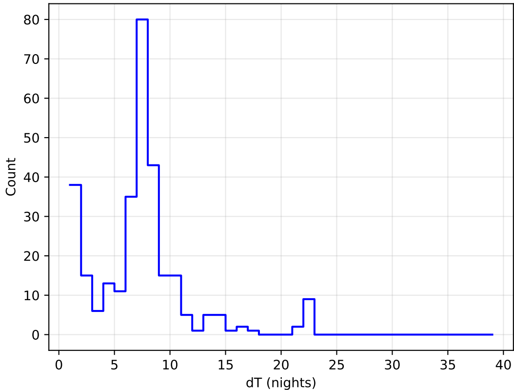
too_elab_r32_d3_ugrizy_v3.4_10yrs all bands: DD:EDFS Delta Nights Histogram
